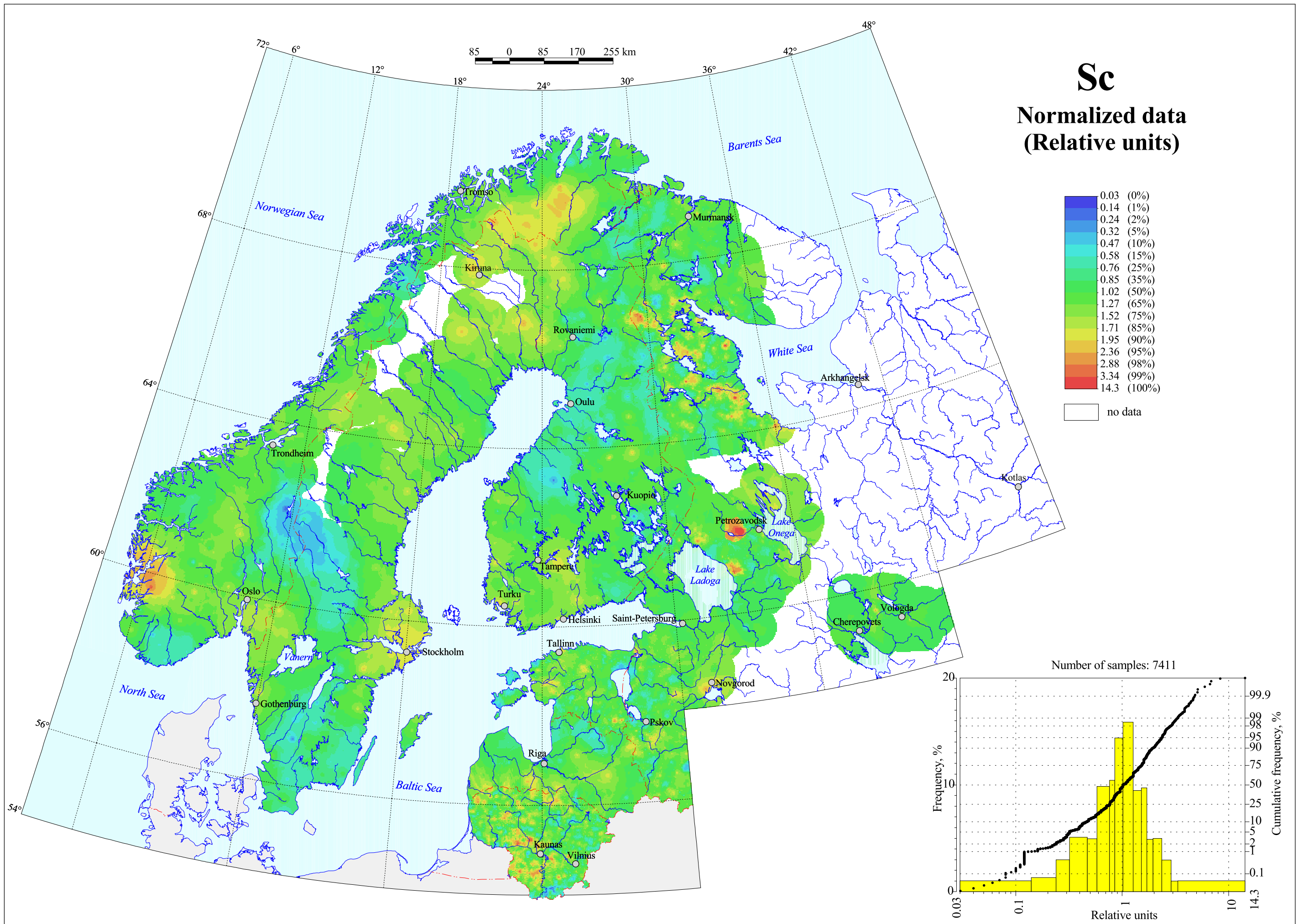
Scandium in Topsoil
